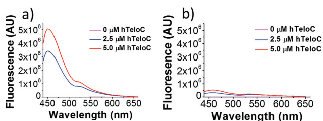
Fig. 1 Fluorescence emission of TO (5 μM) in the presence of 0–5 μM hTeloC in 10 mM sodium cacodylate buffer at pH 5.5 (a) and pH 7.4 (b).
