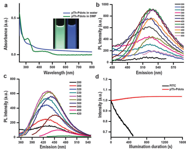
Fig. 2 (a) UV-Vis spectra of pTh-Pdots in DMF and pTh-Pdots in water. Inset shows the optical images under UV illumination at 365 nm. (b) PL emission spectra of pTh-Pdots in DMF at different excitation wavelengths. (c) PL emission spectra of pTh-Pdots in water, (d) photo-bleaching of FITC dye molecules and pTh-Pdots under confocal imaging.
