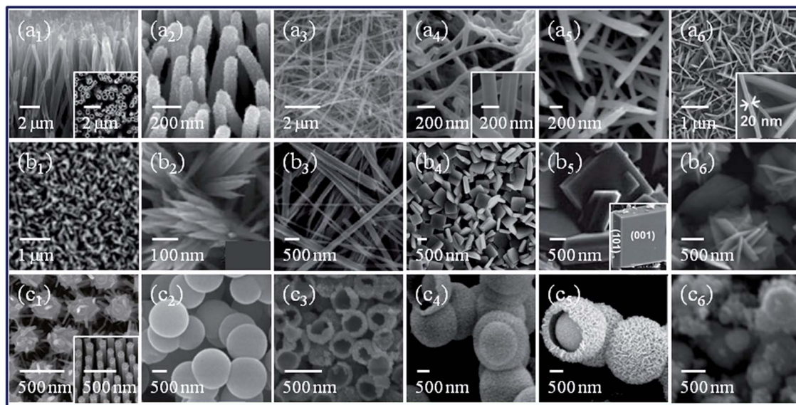
Fig. 11 SEM micrographs of anatase-TiO 2 nanostructures: (a 1 and a 2 ) nanotubes, (a 3 and a 4 ) nanofibres, (a 5 ) nanorods, (a 6 ) nanorods with nanoflakes, (b 1 ) nanoribbon arrays, (b 2 ) nanowires, (b 3 ) nanosheets, (c 1 ) 3D network, (c 2 ) nanospheres, (c 3 ) nanospheres, (c 4 and c 5 ) nanoparticles and (c 6 ) nanoparticles. Insets (a 1 , a 4 , a 6 , b 5 and c 1 ) provide the corresponding higher magnification images. Ref: [a 1 , a 2 ], 50 [a 3 ], 329 [a 4 ], 50 [a 5 ], 269 [a 6 ], 270 [b 1 ], 330 [b 2 ], 271 [b 3 ], 50 [b 4 ], 292 [b 5 ], 41 [b 6 ], 331 [c 1 ], 50 [c 2 ], 274 [c 3 ], 274 [c 4 , c 4 and c 5 ], 273 [c 6 ]. 275 (a 1 , a 2 , a 4 , b 3 and c 1 ) are reprinted with permission from ref. 50. Copyright 2014. American Chemical Society. (a 3 ) is reprinted with permission from ref. 329. Copyright 2005. Elsevier. (a 5 ) is reprinted with permission from ref. 269. Copyright 2013. The Royal Society of Chemistry. (a 6 ) is reprinted with permission from ref. 270. Copyright 2012. The Royal Society of Chemistry. (b 1 ) is reprinted with permission from ref. 330. Copyright 2004. The Royal Society of Chemistry. (b 2 ) is reprinted with permission from ref. 271. Copyright 2011. American Chemical Society. (b 4 ) is reprinted with permission from ref. 292. Copyright 2009. American Chemical Society. (b 5 ) is reprinted with permission from ref. 41. Copyright 2009. American Chemical Society. (b 6 ) is reprinted with permission from ref. 331. Copyright 2011. John Wiley and Sons. (c 2 , c 4 and c 5 ) are reprinted with permission from ref. 273. Copyright 2007. American Chemical Society. (c 3 ) is reprinted with permission from ref. 274. Copyright 2013. The Royal Society of Chemistry. (c 6 ) is reprinted with permission from ref. 275. VBRI Press.
