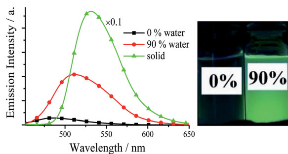
Fig. 2 Emission spectra and photographs (under 360 nm UV light) of 3,5-Cl-Cy in MeCN–H 2 O with different f values ( 1.0 \times 10^{-5} mol dm -3 ) and solid.
