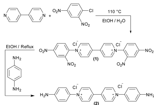
Scheme 1 Synthesis of the viologen derivative 1,1'-bis(4-amino-phenyl)-[4,4'-bipyridine]-1,1'-dium chloride (2).
