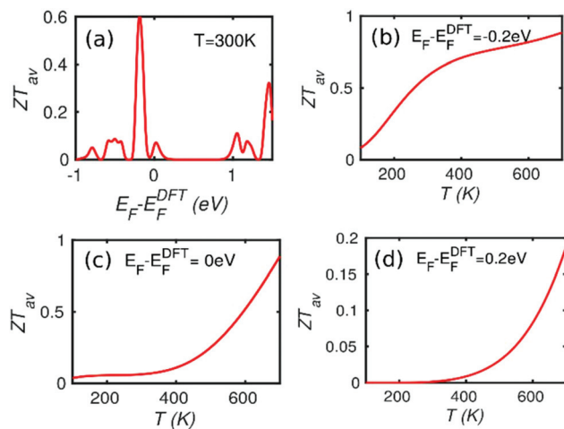
Fig. 6 (a) The ensemble average of the total thermoelectric figure of merit at 300 K for the configurations with p-type dopants Nb replacing Mo atoms in ESI Fig. S9.† (b)–(d) The ensemble average of the total thermoelectric figure of merit as the function of temperature when E_F - E_F^{\text{DFT}} = -0.2 eV, E_F - E_F^{\text{DFT}} = 0 eV, E_F - E_F^{\text{DFT}} = 0.2 eV for the configurations with p-type dopants Nb replacing Mo atoms in ESI Fig. S9.†
