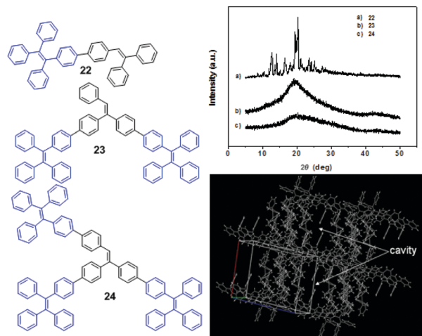
Fig. 3 (top) Wide-angle X-ray diffraction curves of the as-synthesized samples 22–24 ; (bottom) molecular packing of 22 in the single crystal state (wireframe style). (left) The molecular structures of compounds 22–24 . Reproduced with permission from ref. 45. Copyright 2011 Wiley-VCH.
