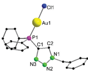
Fig. 1 Molecular structure of 6 in the solid state. Non-coordinating solvents ( \text{CH}_2\text{Cl}_2 , thf) and hydrogen atoms are not displayed. Selected bond lengths [Å] and angles [°]: Au1–Cl1 2.270(3), Au1–P1 2.213(3), C1–C2 1.39(2), P1–Au1–Cl1 177.84(10), P1–C1–N3 124.1(8), P1–C1–C2 127.5(8).
