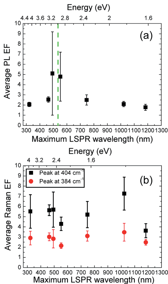
Fig. 4 (a) Average PL peak intensity EF of monolayer MoS 2 as a function of the LSPR position of Ga NPs. The green line represents the laser wavelength, 532 nm. (b) Average Raman EF of monolayer MoS 2 peaks at 384 and 404 cm -1 as a function of the LSPR position of Ga NPs. Error bars indicate the standard deviation.
