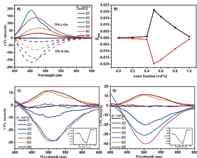
Fig. 4 CPL spectra of (A) TPE-L-Glu and TPE-D-Glu , (D) trans - TPE-L-DGlu in THF/water mixed solvents. Concentration: 1 \times 10^{-5} M; excitation wavelength: 340 nm. (B) g_{lum} versus f_w of TPE-L-Glu and TPE-D-Glu . Inset: g_{lum} versus f_w of cis - TPE-L-DGlu and trans - TPE-L-DGlu .
