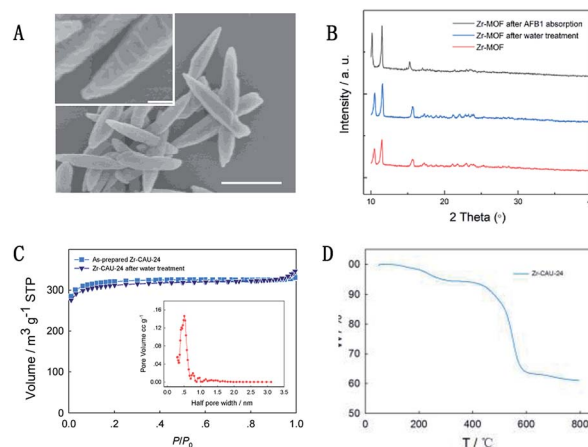
Fig. 2 Scanning electron microscopy images of prepared Zr-CAU-24 crystals with different magnification times. Scale bar: 1 \mu\text{m} (A), (inset). PXRD of Zr-CAU-24 crystals before and after water treatment and AFB1 absorption, (B) and \text{N}_2 adsorption/desorption isotherms (C) of Zr-CAU-24 crystals before and after 24 h water treatment. TGA result of as-prepared Zr-CAU-24 crystals (D).
