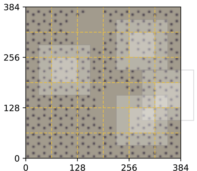
Fig. 4 Decomposition of input image for the quantum mechanical density functional theory calculation using f = 64 and c = 32 . Four tiles consisting of a focus region and context region are highlighted. Overlap in the context region is by design and the EDNN must learn to ignore this overlap in the final reduction of the extensive quantity.
