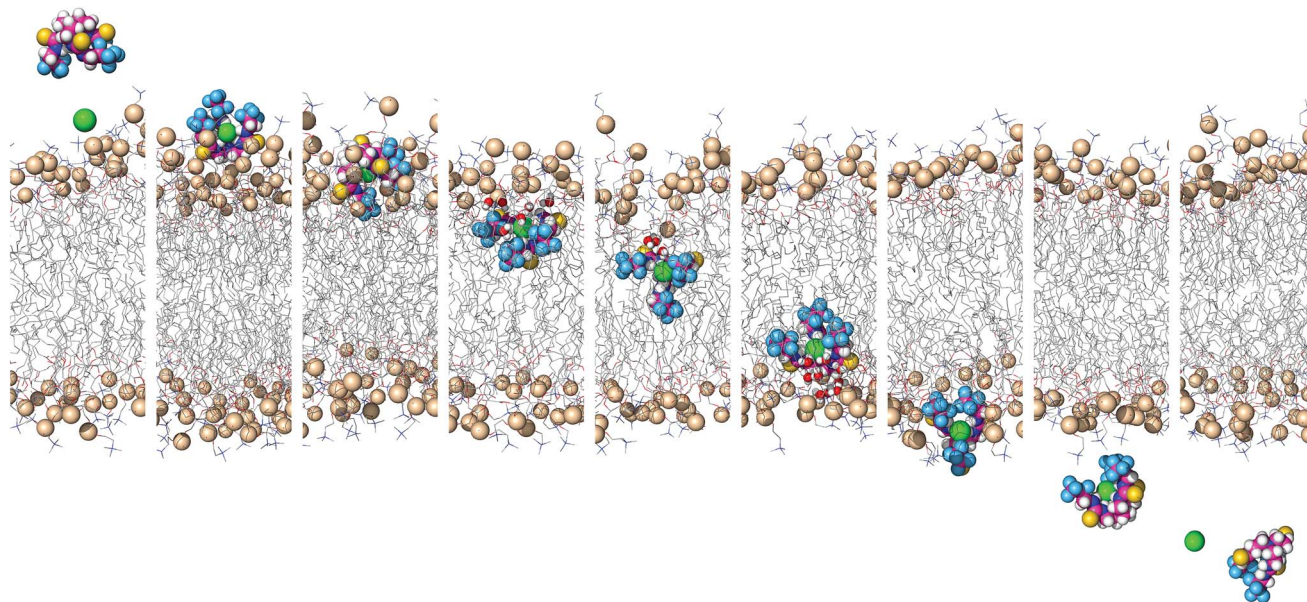
Fig. 9 Consecutive snapshots depicting the movement of 6 across the POPC bilayer in a 170 ns long SMD simulation. The free transporter binds \text{Cl}^- before permeating and crossing the bilayer to the opposite side, where the anion dissociates from the transporter. For further caption details, see Fig. 8.
