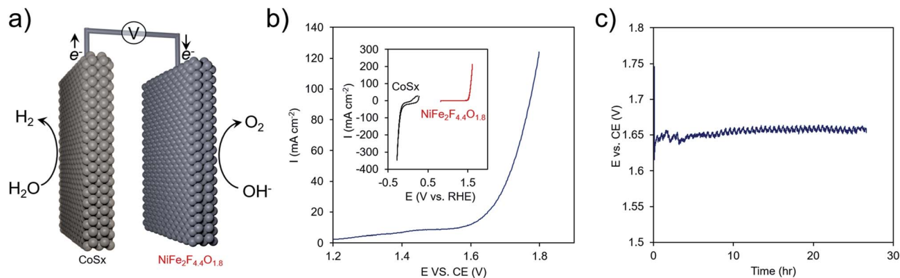
Fig. 8 (a) Overall water electrolysis with \text{NiFe}_2\text{F}_{4.4}\text{O}_{1.8} as the anode. (b) A \text{NiFe}_2\text{F}_{4.4}\text{O}_{1.8} was integrated with a \text{CoS}_x cathode to put together an overall water electrolysis system comprised of earth-abundant materials. (c) This system featured an onset of \sim 1.60 V and required \sim 1.65 V to generate a stable current of 10 \text{ mA cm}^{-2} .
