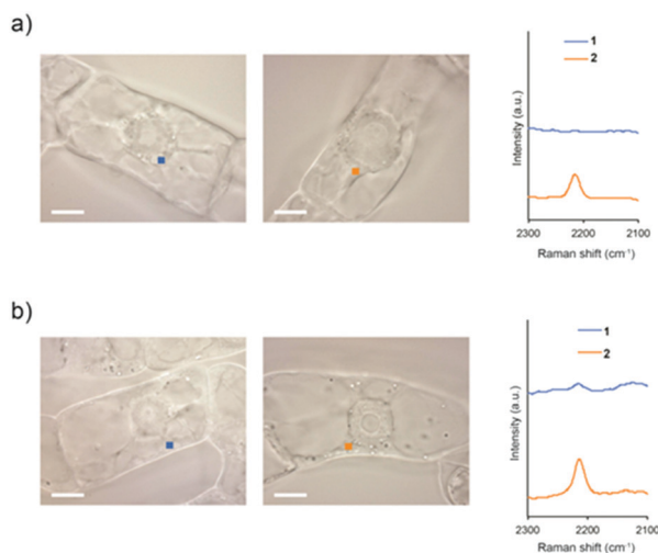
Fig. 4 Raman spectra of BY-2 cells in the cytoplasm. (a) The cells were treated with 1 or 2 at 4 °C. (b) The cells were treated with 1 or 2 in the presence of Wortmannin. The spectra were obtained after 5 h of treatment with 100 \mu\text{M} 1 or 2 . The cytoplasm area in BY-2 cells (1 \mu\text{m} \times 1 \mu\text{m} in size) used for obtaining the averaged Raman spectra are presented by squares in the images. Scale bars are 10 \mu\text{m} .
