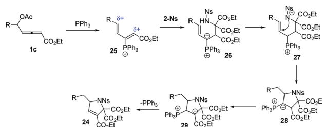
Scheme 8 Plausible mechanisms.
