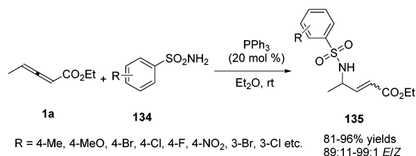
Scheme 43 Phosphine-catalysed \gamma -umpolung additions of sulphonamides to c -substituted allenolates.
