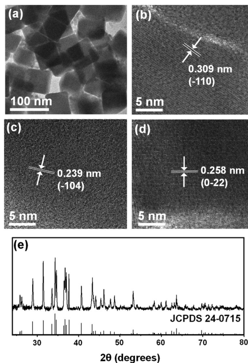
Fig. 3 (a) TEM image of Ag 2 S nanocubes obtained at 72 h and (b–d) their HR-TEM images showing d -spacing of (−110), (−104), and (0−22) crystal facets. (e) XRD pattern of the Ag 2 S nanocubes.
