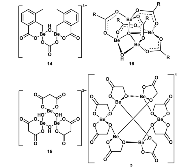
Fig. 8 Multinuclear beryllium compounds with bio-relevant ligands, which all contain six- or eight-membered beryllium heterocycles ( \text{R} = 2\text{-F-C}_6\text{H}_4 ). 39,41,57,58
