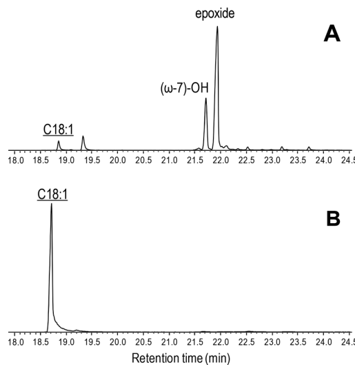
Fig. 5 GC-MS comparison of the reactions of C. virescens UPO (A) and its T158F variant (B) with oleic acid. Peaks of hydroxy and epoxy derivatives are shown, together with the remaining substrate (underlined). The small peak after the substrate is a fatty-acid impurity. See Fig. 2 for the reaction conditions and Table 2 for peak quantification.
