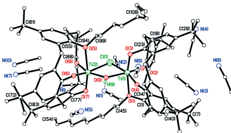
Fig. 7 Molecular structure of \{[\text{Ti}(\text{L})(\text{O})_3(\text{On-decyl})_2(\mu\text{-Cl})(\mu\text{-OH})]\cdot 8.5\text{MeCN}\} (10·8.5MeCN) (most H atoms are omitted for clarity). Selected bond lengths (Å) and angles (°): Ti(1)–O(1) 2.381(3), Ti(1)–O(2) 1.817(3), Ti(1)–O(3) 1.852(3), Ti(1)–O(4) 1.793(3), Ti(1)–O(9) 2.000(3), Ti(1)–Cl(1) 2.5177(14); O(1)–Ti(1)–O(3) 168.54(13), O(2)–Ti(1)–O(4) 102.84(15), Cl(1)–Ti(1)–O(9) 74.82(10), Ti(1)–O(1)–C(1) 112.8(2), Ti(1)–O(2)–C(12) 150.5(3), Ti(1)–O(3)–C(23) 119.9(2), Ti(1)–O(4)–C(34) 168.3(3).
