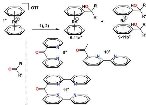
Scheme 5 Reaction scheme for conjugation of polypyridyl ligands to [\text{Re}(\eta^6\text{-C}_6\text{H}_6)_2](\text{OTf}) . Reaction conditions: (1) Lithiation/deprotonation 3.0 eq. of LDA, 1.5 h, -78^\circ\text{C} , THF; (2) addition to carbonyl 5 h, -78^\circ\text{C} , THF.
