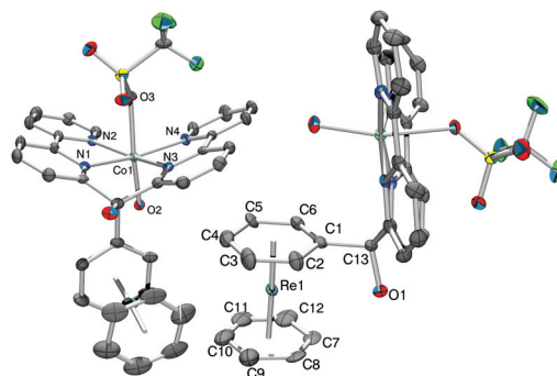
Fig. 3 ORTEP representation of the crystal structure of [12\text{a}]\text{OTf} along two different views. Hydrogen atoms and two OTf-anions have been omitted for clarity; thermal ellipsoids represent 40% probability. Selected bond lengths (Å): \text{Re1}-\text{C1} 2.252(8), \text{Re1}-\text{C2} 2.235(9), \text{Re1}-\text{C3} 2.218(10), \text{Re1}-\text{C4} 2.244(10), \text{Re1}-\text{C5} 2.259(10), \text{Re1}-\text{C6} 2.228(9), \text{Re1}-\text{C7} 2.228(10), \text{Re1}-\text{C8} 2.198(10), \text{Re1}-\text{C9} 2.206(13), \text{Re1}-\text{C10} 2.206(13), \text{Re1}-\text{C11} 2.238(11), \text{Re1}-\text{C12} 2.226(12), \text{C1}-\text{C13} 1.550(11), \text{N1}-\text{C01} 2.100(7), \text{N}-\text{C01} 2.108(7), \text{N3}-\text{C01} 2.103(7), \text{N4}-\text{C01} 2.109(7), \text{Co1}-\text{O2} 2.064(6), \text{Co1}-\text{O3} 2.279(6).
