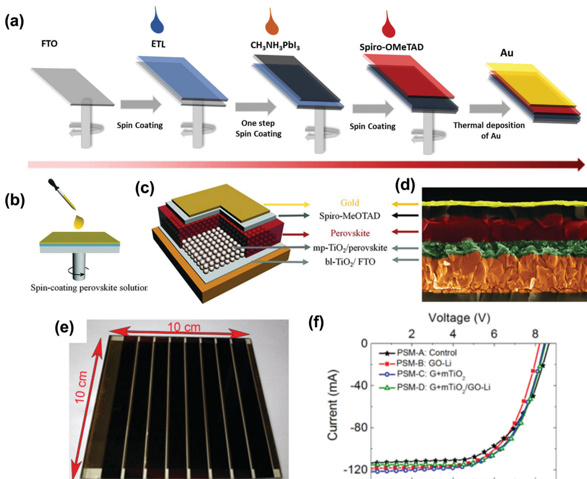
Fig. 3 Perovskite film deposition and device structure. (a) Schematic of the perovskite solar devices step by step. (b) Schematic showing the spin coating of the perovskite solution on the substrate. (c) Schematic of the perovskite solar cell configuration, where a smooth and compact perovskite capping layer fully covers the mesoporous TiO 2 layer (mp-TiO 2 ) infiltrated with perovskites. (d) A high-resolution cross-sectional SEM image of a complete perovskite solar cell with large area fabricated by the spin coating technique. (b–d) Reproduced with permission from ref. 61. Copyright © 2016 SpringerNature. (e) Photograph of the large-area perovskite solar module (50 cm 2 active area). (f) Current–voltage ( I – V ) characteristics of tested modules (i.e., PSM-A, PSM-B, PSM-C, and PSM-D). All the I – V measurements refer to the encapsulated devices. (e and f) Reproduced with permission from ref. 62. Copyright © 2016 American Chemical Society.
