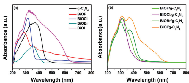
Fig. 8 DRS plots of (a) BiOX and g\text{-C}_3\text{N}_4 and (b) BiOX/ g\text{-C}_3\text{N}_4 composites (X = F, Cl, Br and I).
