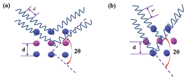
Fig. 6 Schematic illustration of XRD for the structural transformation of the \text{CH}_3\text{NH}_3\text{PbI}_3 perovskite.
