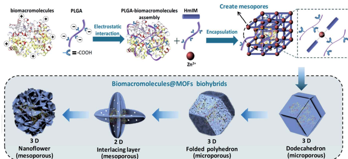
Fig. 3 Illustration of the deformable MOF by using a PLGA modulator. Reproduced from ref. 41 with permission of WILEY-VCH Verlag GmbH & Co. KGaA, Weinheim.
