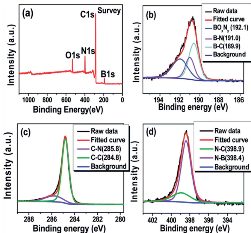
Fig. 8 Example of XPS spectra that are deconvoluted to show B-N, B-C, C-N, C-C etc. bonds for a h-BN coated MWCNT synthesized via a B 2 O 3 + NH 3 pathway using H 3 BO 3 and CO(NH 2 ) 2 as starting precursors. (a) XPS survey spectrum (b–d) High resolution spectra of B1s, C1s and N1s respectively. Reproduced from ref. 34 with permission from the Royal Society of Chemistry.
