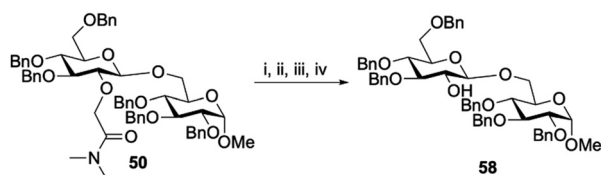
Scheme 1 Removal of the auxiliary. Reagents and conditions (i) \text{H}_2\text{O} (2.2 eq.), t\text{-BuOK} (5.9 eq.), THF, rt; (ii) \text{DIPEA} (1.2 eq.), \text{DPPA} (1.1 eq.), DMF, 0^\circ\text{C} - rt; (iii) t\text{-BuOH} , DMF, 100^\circ\text{C} ; (iv) \text{NaOH} , THF, EtOH, 60^\circ\text{C} .
