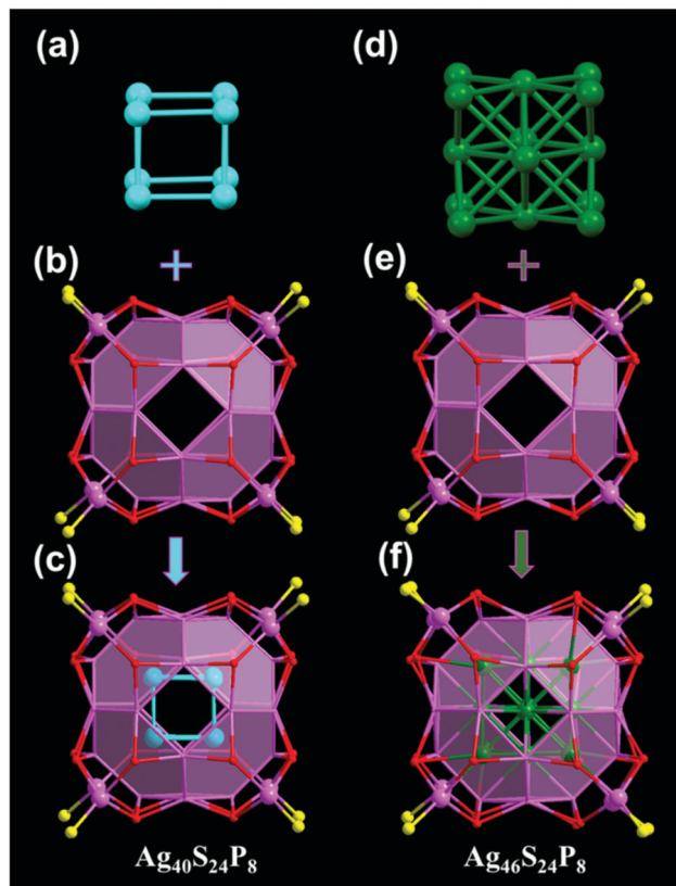
Fig. 8 Core, shell and framework of Ag 40 (2,4-DMBT) 24 (PPh 3 ) 8 and Ag 46 (2,5-DMBT) 24 (PPh 3 ) 8 . Adapted with permission from ref. 73. Copyright 2018, American Chemical Society.
