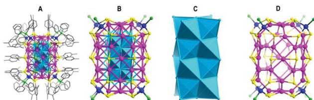
Fig. 7 (A) Total structure of Ag 67 (SPhMe 2 ) 32 (PPh 3 ) 8 . (B) The structure of Ag 67 S 32 P 8 obtained by disconnecting carbon atoms in A. (C) Ag 23 metal core. (D) The structure of the NC without the Ag 23 metal core, i.e. , Ag 44 (SPhMe 2 ) 32 (PPh 3 ) 8 . Adapted with permission from ref. 75. Copyright 2017, American Chemical Society.
