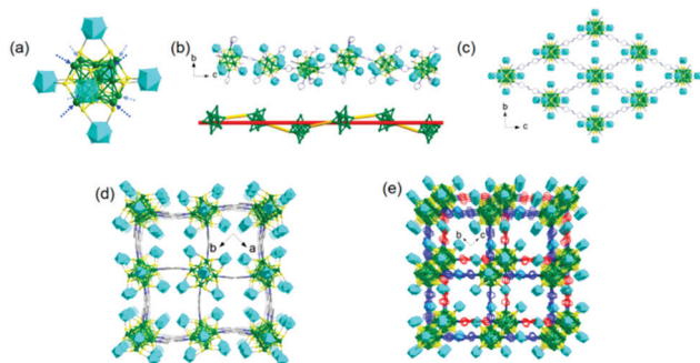
Fig. 6 Structural representation of the (a) 1,2-dithiolate- o -carborane-capped Ag 14 NC; (b) 1D helix; (c) 2D grid network; (d) 3D porous framework and (e) 2-fold interpenetrated porous 3D frameworks. Adapted with permission from ref. 72. Copyright 2018, American Chemical Society.
