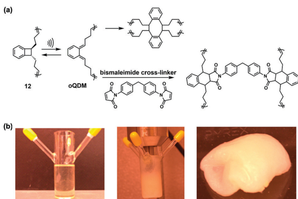
Fig. 13 (a) Two crosslinking pathways of oQDM intermediates generated through ring-opening of BCBs in polymer 12 under pulsed ultrasonication. (b) Solution of 25 \text{ mg mL}^{-1} 12 + bismaleimide cross-linker before (left) and after (middle) sonication and following removal from the Suslick vessel (right). Reproduced with permission. 51 Copyright 2015, American Chemical Society.
