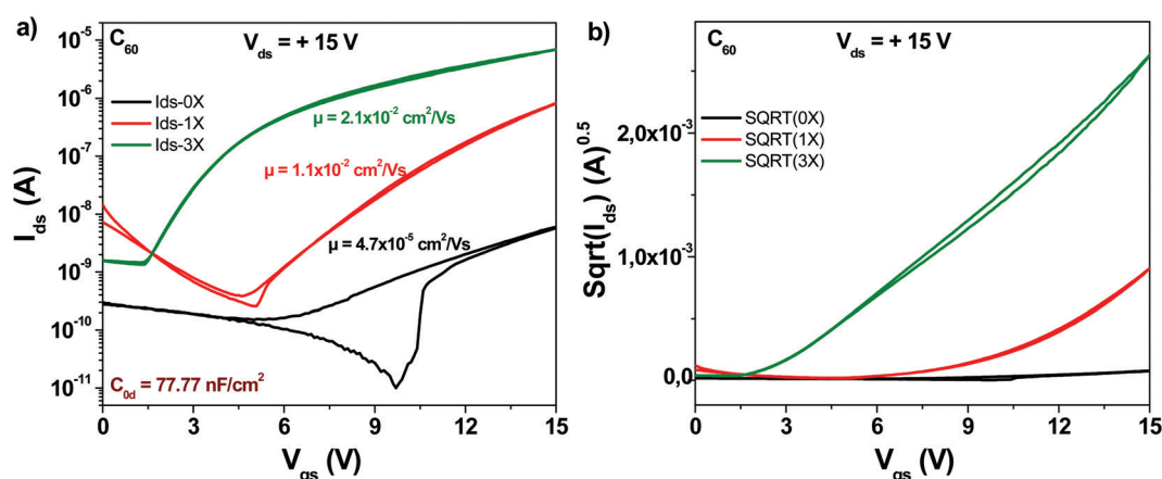
Fig. 5 (a) Comparison of OFET devices with three different grades of fullerene ( C_{60} ) semiconductor purity: unpurified (0 \times in graph legend), one time purified (1 \times in graph legend) and three times purified respectively (3 \times in graph legend); (b) the \sqrt{I_{ds}} vs. V_{gs} of the three purity grades presented in panel (a).
