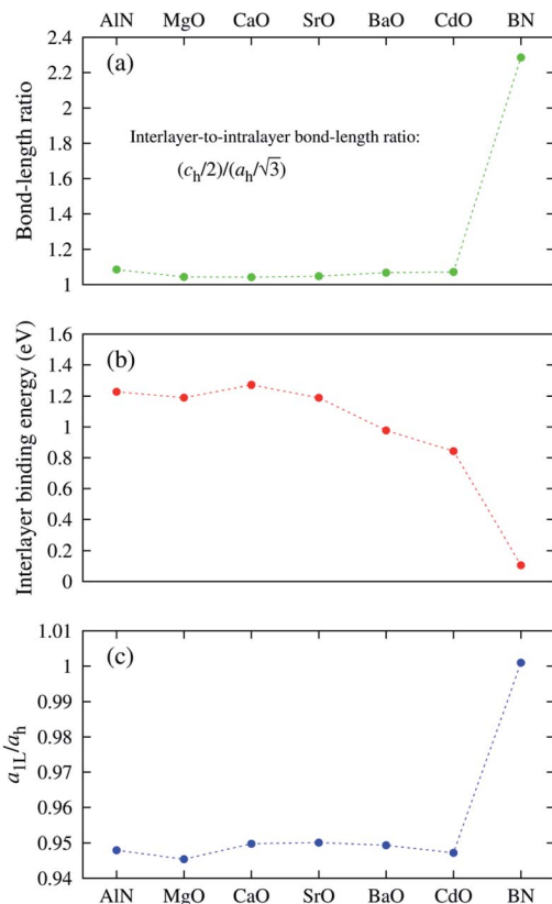
Fig. 2 Structural features of the h-MgO structure in contrast to those of h-BN. (a) Ratios of the interlayer distance ( c_{IL}/2 ) to intralayer bond length ( a_{IL}/\sqrt{3} ). (b) Interlayer binding energies, defined as monolayer-to-bulk total energy difference per cation-anion pair. (c) Monolayer-to-bulk lattice parameter ratios ( a_{1L}/a_h ).
