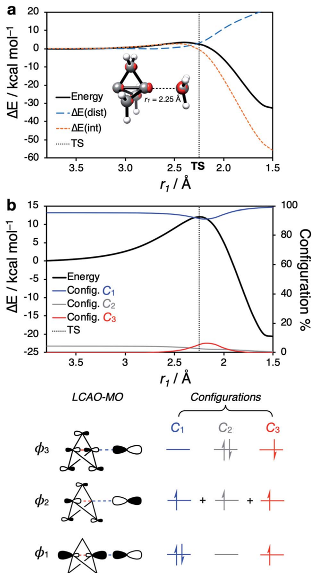
Fig. 5 (a) PES (DLPNO-CCSD(T)/def2-QZVPP//CASCF(3,3)/def2-QZVPP) and distortion/interaction energies for the addition of \cdot\text{CH}_3 to 1 . (b) (Top) PES (CASCF(3,3)/def2-QZVPP) for the addition of a methyl radical to 1 , showing the proportion of each leading electronic configuration as a function of the forming C–C bond ( r_1 ). (Bottom) LCAO-MO depiction of the frontier molecular orbitals involved in the radical addition process to 1 , and the leading electronic configurations for the reaction.
