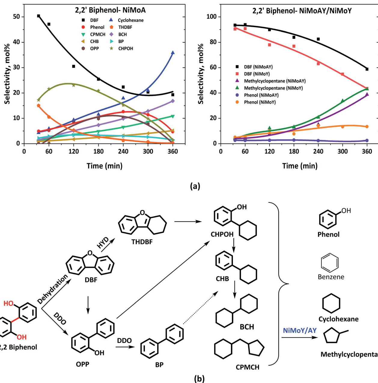
Fig. 4 (a) Product selectivity's during HDO of 2,2'-biphenol over NiMoA, NiMoAY and NiMoY and (b) proposed reaction scheme during HDO of 2,2'-biphenol.
