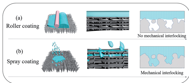
Fig. 1 Schematic diagrams of (a) roller coating, and (b) spray coating to produce thin film polymer composites from incompatible polymers.
