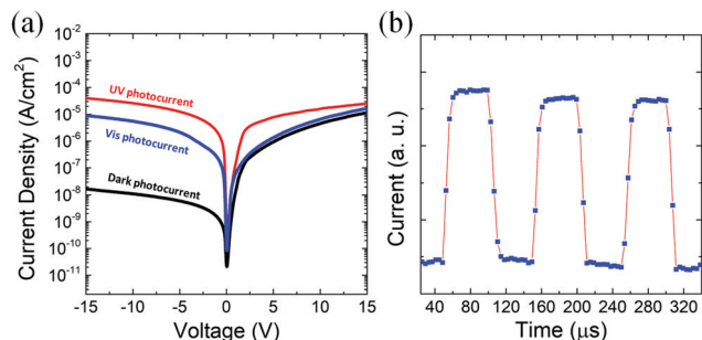
Fig. 2 (a) I - V characteristics of the photodetector measured in the dark, under 760 nm visible illumination, and 375 nm UV illumination. (b) Transient response of the heterojunction photodiode with a rising time of 4.3 \mu s and a falling time of 5.2 \mu s measured under ambient conditions.
