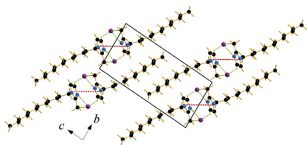
Fig. 5 Packing diagram of \text{C}_{12}\text{C}_1\text{C}_0 . Projection on the bc plane. \text{C}_g - \text{C}_g contacts are shown by red and \text{Br}\cdots\text{H} bonds by green dashed lines.
