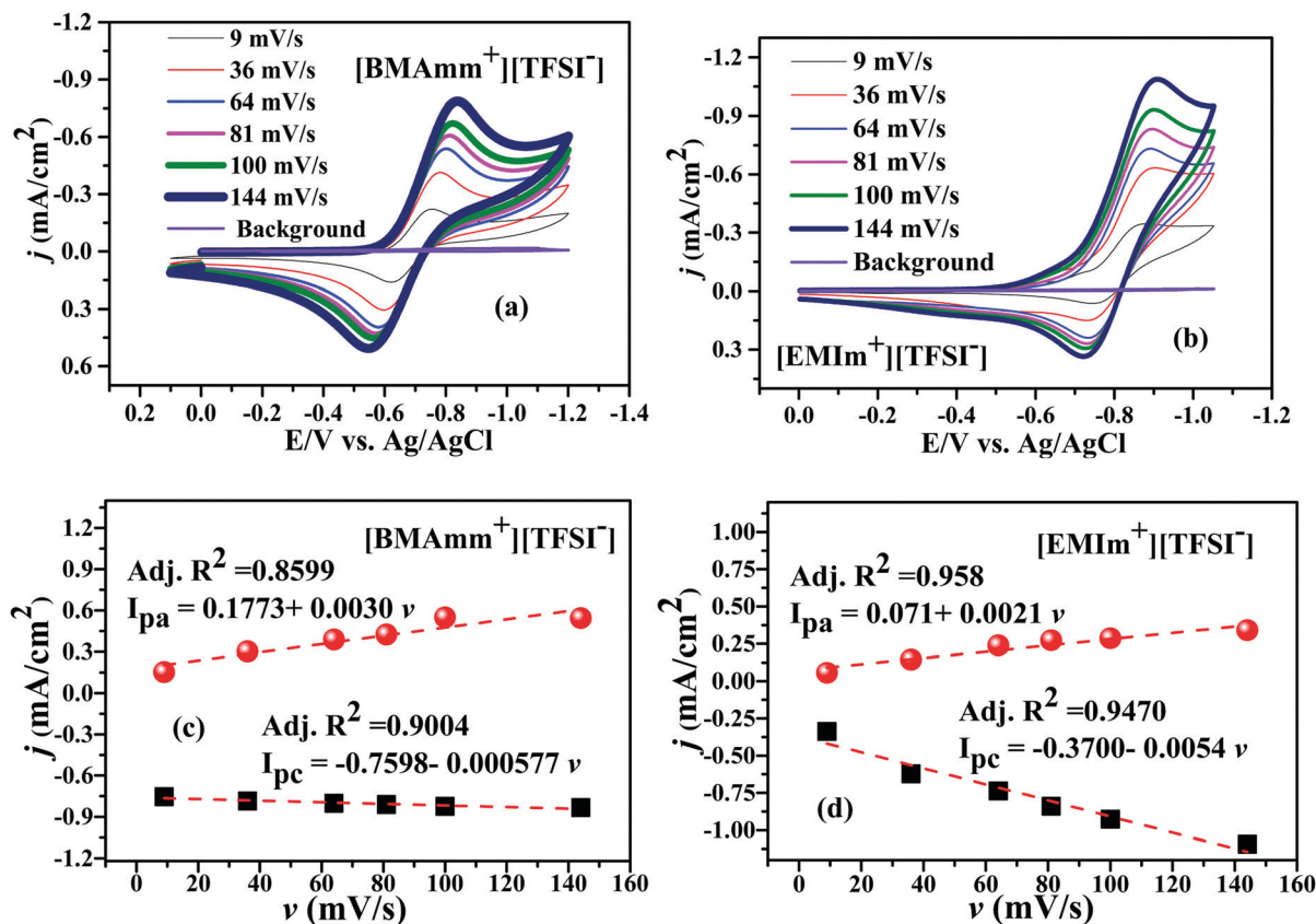
Fig. 3 CVs of \text{O}_2^{\bullet-} generation in (a) [\text{BMAMm}^+][\text{TFSI}^-] and (b) [\text{EMIm}^+][\text{TFSI}^-] , and current density against sweep rate in (c) [\text{BMAMm}^+][\text{TFSI}^-] and (d) [\text{EMIm}^+][\text{TFSI}^-] .
