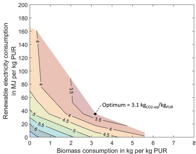
Fig. 4 Pareto frontiers of the global warming impact of 1 kg PUR as a function of biomass and renewable electricity consumption. The biomass supply has a global warming impact of -1.7 \text{ kgCO}_2\text{-eq/kg}_{\text{biomass}} (best case). The electricity supply has a global warming impact of 3 \text{ gCO}_2\text{-eq/kg}_{\text{PUR}} (best case). The black curves show combinations of bio-based and CCU-based production with constant global warming impacts (iso-GWI curves).
