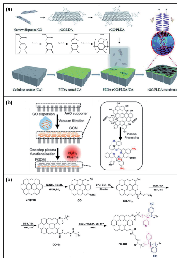
Fig. 8 (a) An illustration of the fabrication of GO membranes using chiral amplification. Adapted with permission from ref. 78. Royal Society of Chemistry, copyright 2020. (b) Left: An illustration of the preparation steps of functionalized graphene oxide (FGO) nanosheets using a one-step plasma processing method. Right: The chemical structure of graphene oxide (GO) nanosheets and plasma FGOMs. Adapted with permission from ref. 79. American Chemical Society, copyright 2021. (c) A schematic illustrating the synthetic pathway of PB-GO. BiBB: 2-bromo-2-methylpropanoyl bromide. Adapted with permission from ref. 80. Elsevier Science Ltd. Copyright 2020.
