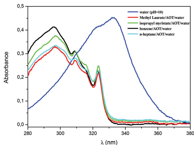
Fig. 3 Absorption spectra for 1-naphthyl phosphate hydrolysis catalyzed by AP in nonpolar solvent/AOT/water RMs, at 35 °C. W_0 = 10 , [AOT] = 0.1 \text{ M} , [1 - \text{naphthyl phosphate}] = 1 \times 10^{-4} \text{ M} . [AP] = 1 \times 10^{-7} \text{ M} . Reaction time = 15 minutes.
