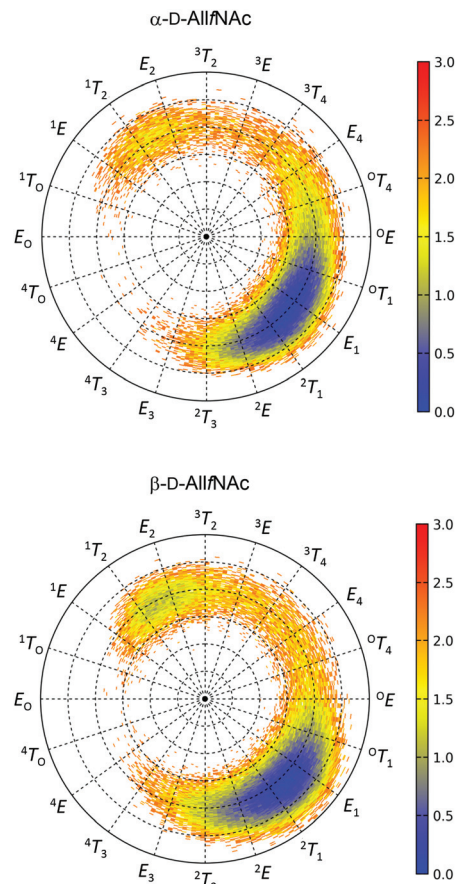
Fig. 2 Two-dimensional free energy maps of (top) \alpha\text{-D-AllfNAc} and (bottom) \beta\text{-D-AllfNAc} . The location at the perimeter corresponds to the pseudorotation phase P whereas the radius of the pseudorotation wheel corresponds to a puckering amplitude \phi_m varying linearly from 0^\circ to 60^\circ . The energy scale is in \text{kcal mol}^{-1} .
