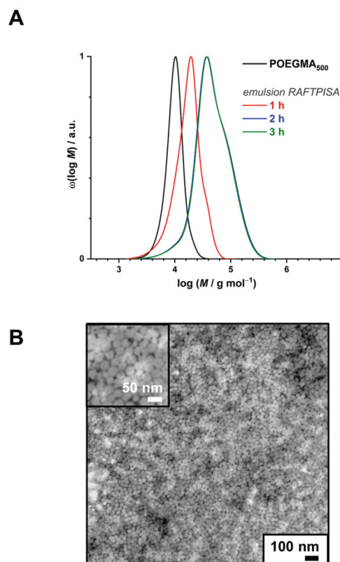
Fig. 2 (A) Size-exclusion chromatograms of polymers obtained by PBBMA emulsion RAFTPISA in water/ethanol 3 : 1 vol/vol at 70 °C with POEGMA 500 at DP_{th} = 100, and 20 wt% solids content (entry 4 from Table S2 † ). (B) Transmission electron micrograph of nanoparticles obtained in the conditions mentioned above, after 2 h.
