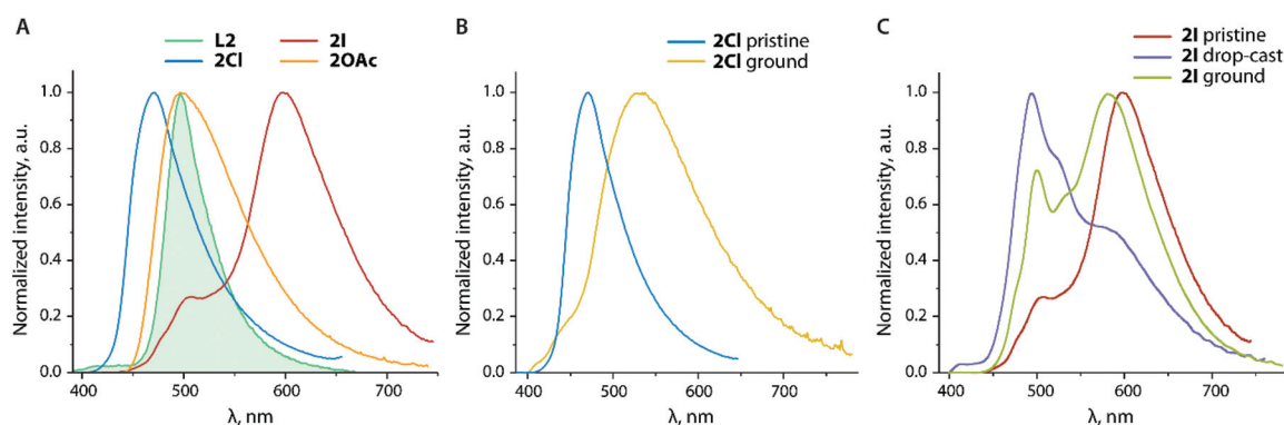
Fig. 9 Normalized solid state emission spectra of (A) L2 (filled graph) and 2X (298 K, \lambda_{\text{exc}} = 400 nm for 2I , \lambda_{\text{exc}} = 350 nm for other samples); (B) pristine and ground 2CI (298 K); and (C) pristine, ground and dropcast 2I (298 K).
