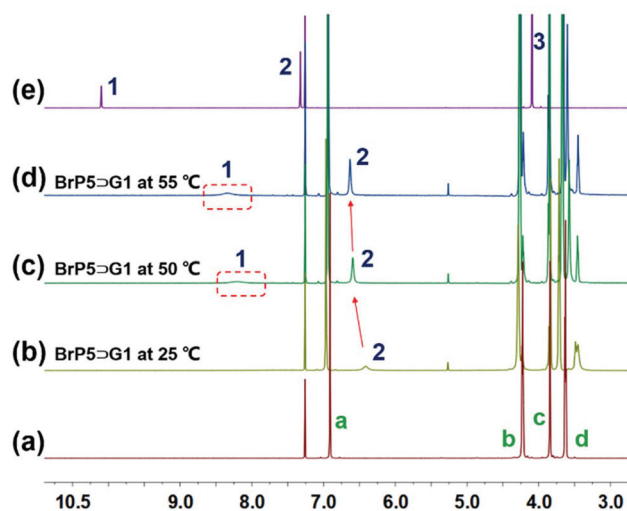
Fig. 5 Partial temperature-dependent ^1\text{H} NMR spectra (600 MHz, \text{CDCl}_3 ): (a) \text{BrP5} at 25 °C; (b) \text{BrP5}\supset\text{G1} at 25 °C; (c) \text{BrP5}\supset\text{G1} at 50 °C; (d) \text{BrP5}\supset\text{G1} at 55 °C; and (e) \text{G1} at 25 °C.
