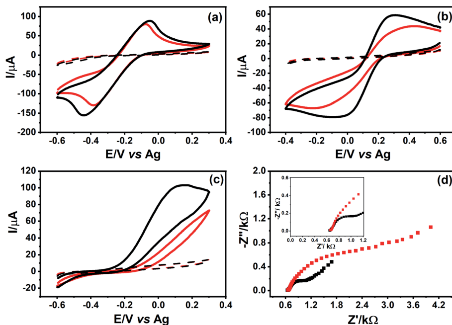
Fig. 5 CVs recorded using (red line) non-treated and (black line) \text{CO}_2 laser-treated PDEs in the absence (dashed line) and presence (solid line) of (a) 5 \text{ mmol L}^{-1} [\text{Ru}(\text{NH}_3)_6]\text{Cl}_3 in 0.1 \text{ mol L}^{-1} \text{ KCl} , (b) 5 \text{ mmol L}^{-1} \text{ K}_3[\text{Fe}(\text{CN})_6] in 0.1 \text{ mol L}^{-1} \text{ KCl} , (c) 5 \text{ mmol L}^{-1} \text{ AA} in 0.1 \text{ mol L}^{-1} \text{ PBS} ( \text{pH} = 6.8 ), and (d) Nyquist plot recorded in both PDEs in a mixture of 5 \text{ mmol L}^{-1} potassium ferricyanide/ferrocyanide solution in 0.1 \text{ mol L}^{-1} \text{ KCl} solution. The frequency range is from 10^5 to 10^{-2} Hz. Scan rate used to record the CVs was 10 \text{ mV s}^{-1} .
