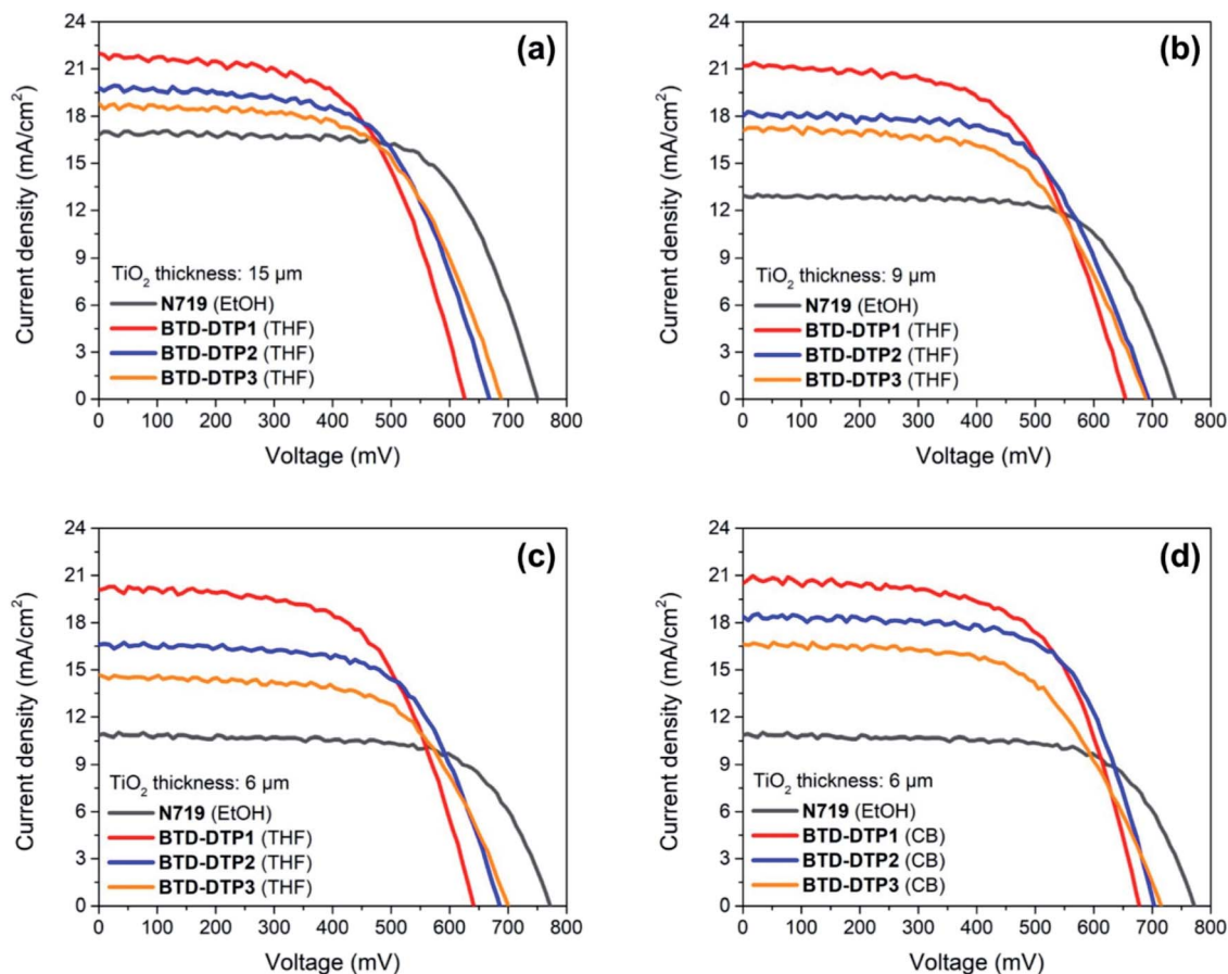
Fig. 6 J - V curves of the solar cells that employed working electrodes of different thicknesses sensitized by organic dyes BT-DTP1–3 as well as Ru-dye N719. (a) 15 \mu\text{m} , THF solution; (b) 9 \mu\text{m} , THF solution; (c) 6 \mu\text{m} , THF solution; (d) 6 \mu\text{m} , CB solution.
