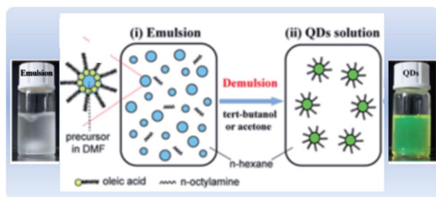
Fig. 10 Illustration of the emulsion synthesis method and photographs of the \text{MAPbBr}_3 emulsion and the resultant colloidal solution upon addition of the demulsifier. Modified with permission from ref. 162.
