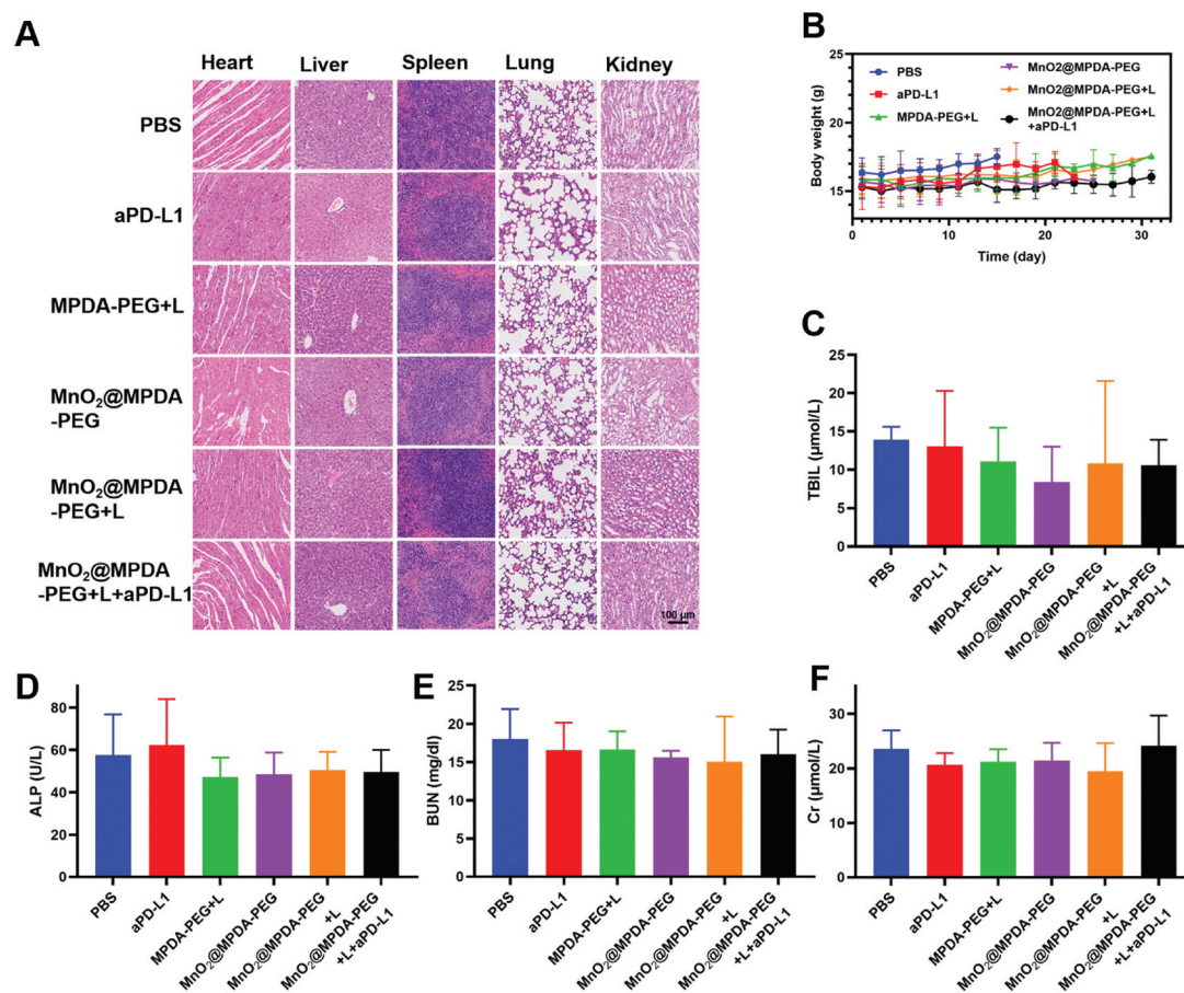
Fig. 5 Systematic toxicity analysis. (A) H&E staining of major organs from the mice with different treatments. Scale bars: 100 \mu\text{m} . (B) Body weight monitoring of the mice during the entire experimental period. (C–F) Blood biochemistry tests including TBIL, ALP, BUN and Cr after various treatments of CT26 tumor-bearing mice at day 10.
