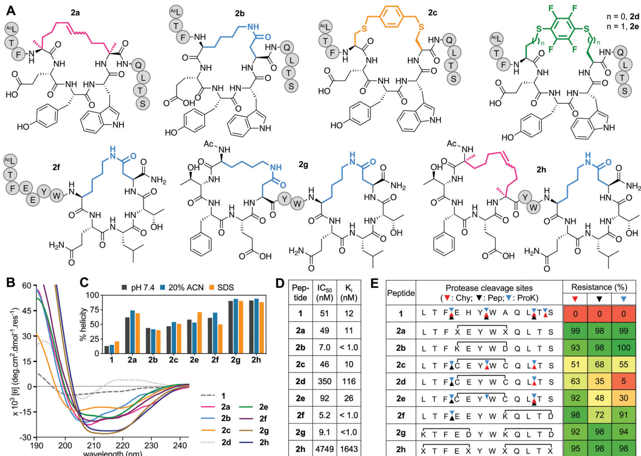
Fig. 2 A. Structures of ( i \rightarrow i + 4 )-crosslinked peptides 2a–h . B. CD spectra for 2a–h vs. 1 (50 \mu M) in 10 mM phosphate buffer (pH 7.4) at 22 ^{\circ} C. C. Percent helicity calculated from CD spectra ( \theta_{220} ) in 10 mM phosphate buffer (pH 7.4), 20% ACN or 20 mM SDS buffer. D. IC 50 = mean peptide concentration for inhibiting 50% binding of 1 -FITC (10 nM) to hDM2 (25 nM) measured by FP. pIC 50 \pm SEM values are reported in Fig. S1 (ESI † ). Binding affinity ( K_i ) calculated from IC 50 values. E. Heatmap indicating percent peptide intact after 2 h incubation with chymotrypsin (Chy), pepsin (Pep) or proteinase K (ProK) at 22 ^{\circ} C at pH 8 or 2 (Pep only), measured by LCMS. Arrows point to respective protease cleavage sites as revealed by LCMS analysis of the cleaved fragments.
