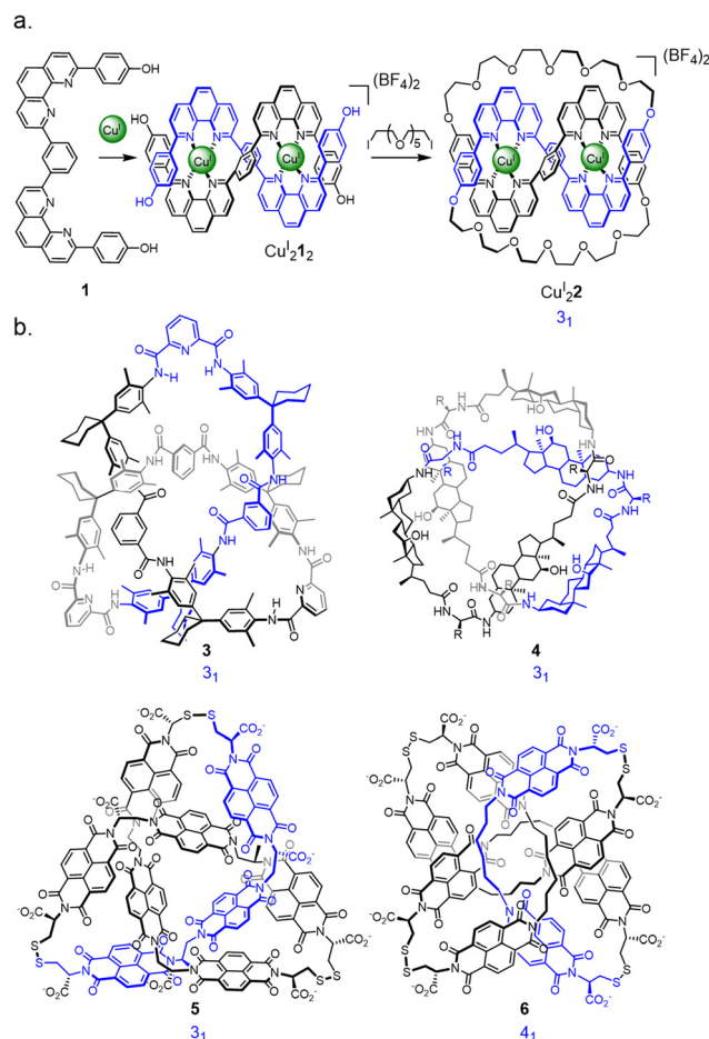
Fig. 2 Early synthetic molecular knots. (a) Coordination of \text{Cu}^I to ditopic ligand 1 to construct trefoil knot \text{Cu}_2^1\text{2} from a linear helicate. 12 (b) Examples of molecular knots discovered through serendipity: Hydrogen bond assembled knot 3 , first prepared by Hunter et al. 31 but structurally re-assigned as a knot following X-ray crystallography by Vögtle et al. 30 Hydrogen bond assembled steroidal knot 4 from Feigel et al. 32 Disulfide-linked trefoil knot 13 5 and figure-eight knot 17 6 discovered by Sanders et al.
